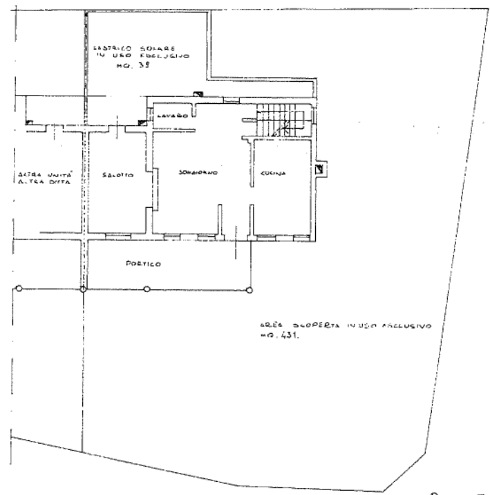
PIANO TERRA H = 2.70 ML
