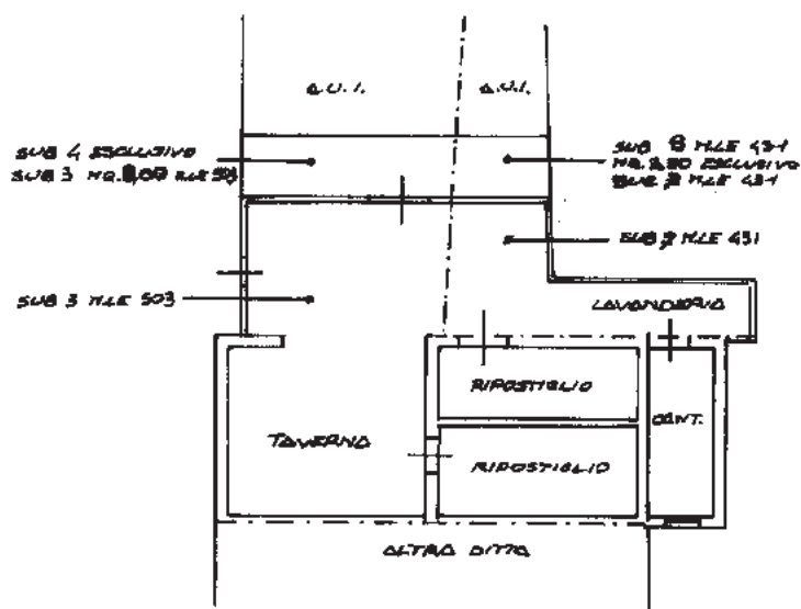
PIANO TERRA h=270
